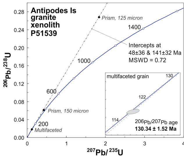
Figure 9. Thermal ionization mass spectrometry U-Pb isotopic age results for single zircon grains from Antipodes Island granite xenolith (Table S3). U-Pb concordia plot shows apparent minor and major reverse discordance for two grains. Maximum age of 130 Ma age is based on the ^{207}\text{Pb}/^{206}\text{Pb} age of the near concordant multifaceted grain, but we report a lower age ^{207}\text{Pb}/^{206}\text{Pb} age of 126 Ma based on likely error in decay constants (see text).
