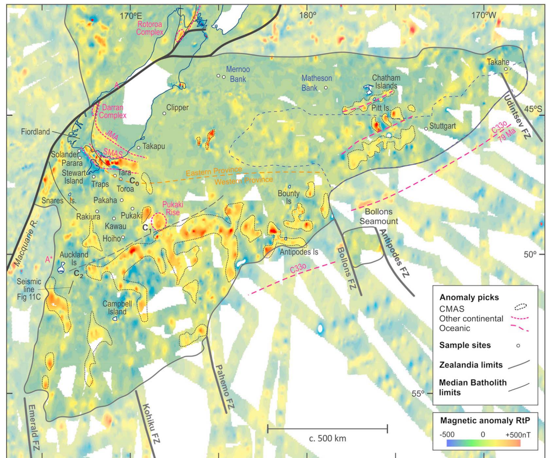
Figure 2. Magnetic map of South Zealandia. Based on Sutherland (1999) and data held by GNS Science. Most of Median Batholith has a much lower magnetic expression than the CMAS (fine black picks), extended herein to include similar anomalies immediately south of Chatham Island. CMAS = Campbell Magnetic Anomaly System; SMAS = Stokes Magnetic Anomaly System; JMA = Junction Magnetic Anomaly. Previous authors (e.g., Sutherland, 1999) have projected Paleozoic-Mesozoic continental margin arc rocks from C_0 to C_1 where it is offset along a putative dextral Campbell Fault (dashed line) to C_2 . HIMU-like basalts dredged from Pukaki Rise are Pliocene in age (Timm et al., 2010) and suggest that at least some of the magnetic rocks within the CMAS are not (directly) related to Late Cretaceous rifting.
