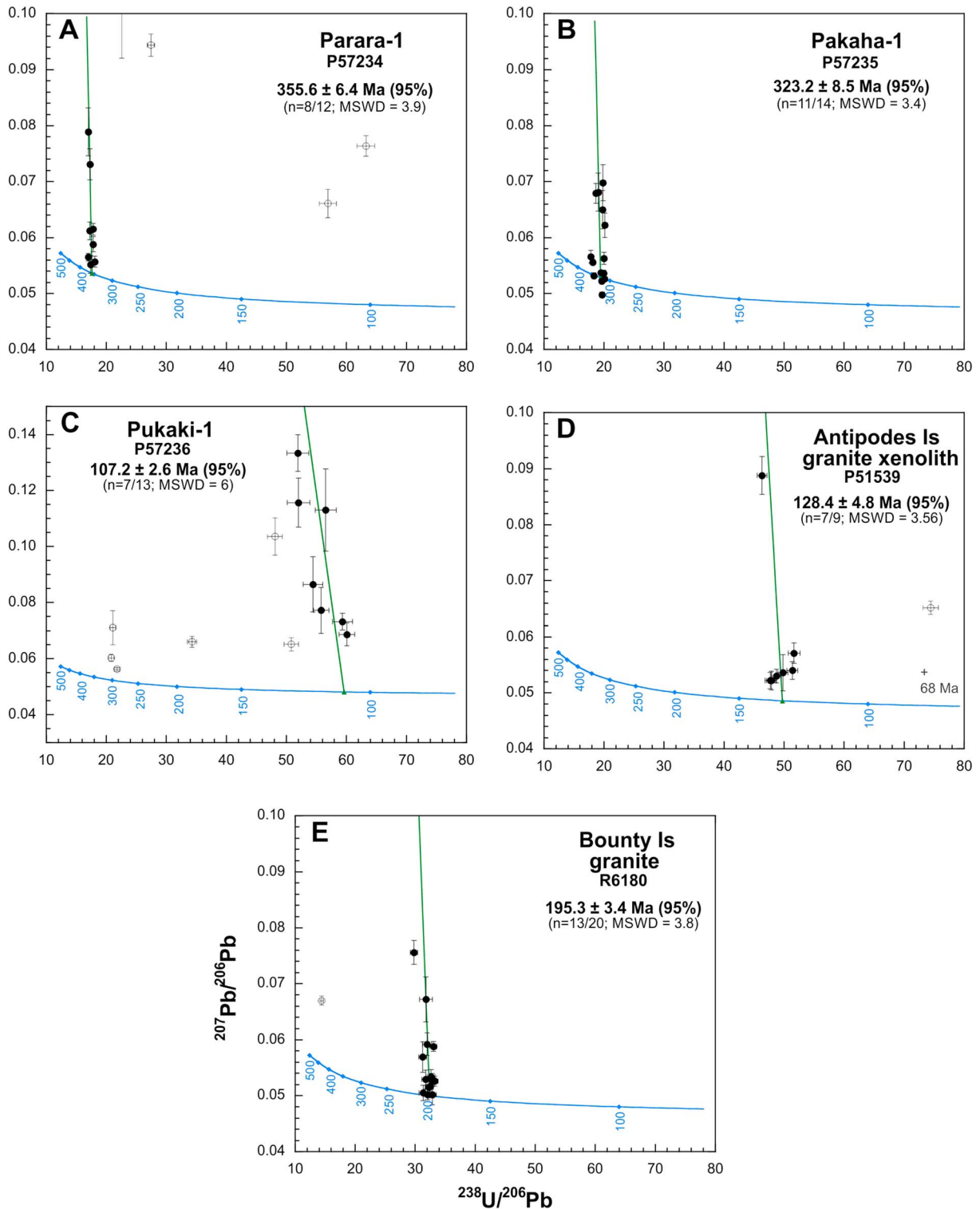
Figure 8. Sensitive high-resolution ion microprobe zircon isotopic data plotted on Tera-Wasserburg concordia plots. Reported age is ^{238}\text{U}/^{206}\text{Pb} intercept of discordia anchored in common lead of Broken Hill composition (Muir et al., 1994). (a–c) Great South Basin well cuttings samples; (d and e) Samples from Antipodes and Bounty Islands, respectively.
