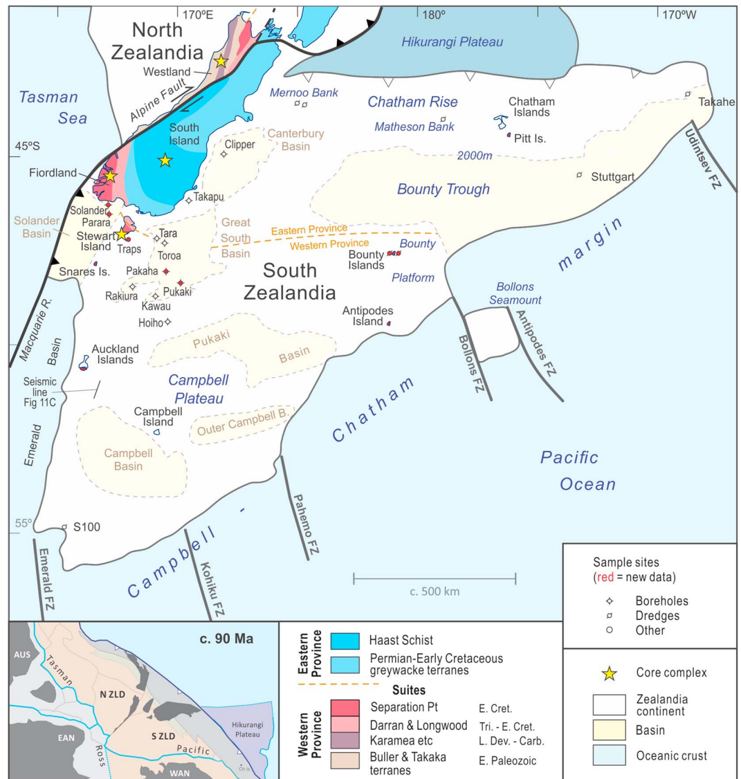
Figure 1. Location map of South Zealandia, highlighting samples used in this study. Inset map shows location of South Zealandia at 90 Ma, within a partly stretched continental ribbon on the SE Gondwana margin (ZLD = proto-Zealandia; WAN = West Antarctica; EAN = East Antarctica; AUS = Australia). Blue lines represent future breakup. Hikurangi oceanic plateau is jammed in a Triassic-Early Cretaceous subduction margin. The Eastern Province comprises terranes representing an accretionary wedge and forearc basin associated with Triassic-Early Cretaceous subduction. Western Province comprises Early Paleozoic metasedimentary terranes, intruded by mid-Paleozoic and Triassic-Early Cretaceous continental margin arc batholiths. Boreholes are detailed in Cook et al. (1999).
