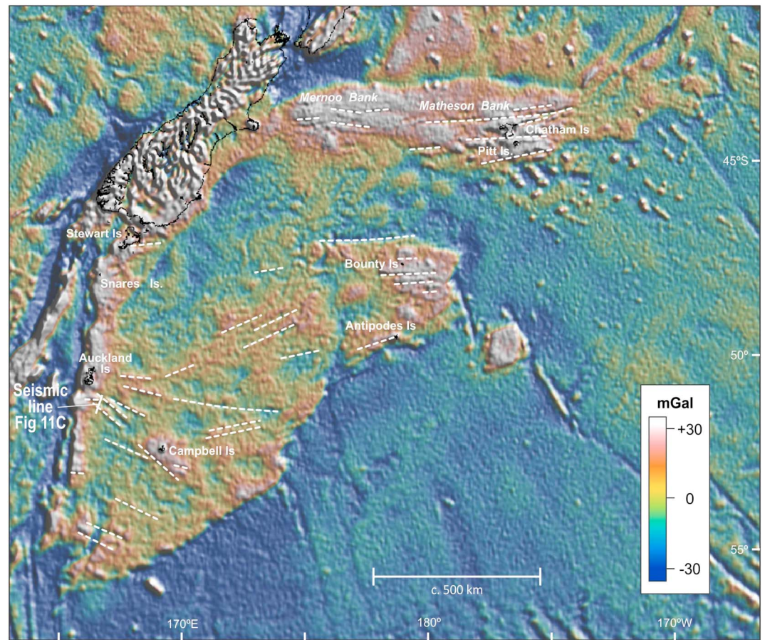
Figure 3. Free-air gravity map of South Zealandia (Sandwell & Smith, 1997) with the most significant linear anomalies, and the location of seismic line 11C, denoted.
